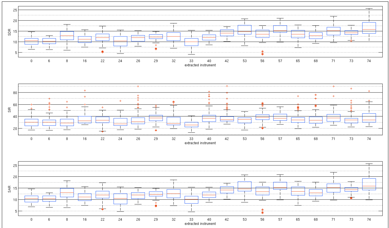
Figure 2. Overall source extraction scores per instrument, mixed with any other instrument. On the x-axis, the MIDI Program Change number. In this and all other figures, standard Matlab style boxplots are used.
